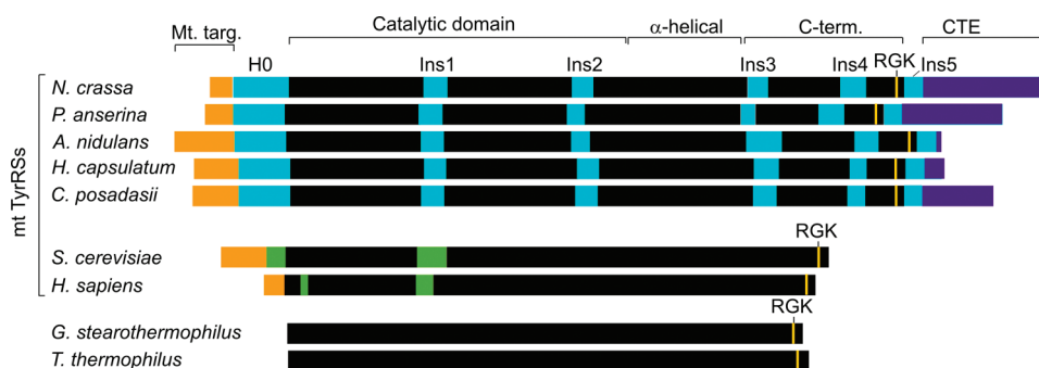
Figure 1. Comparison of splicing-active Pezizomycotina mt TyrRSs with nonsplicing bacterial and mt TyrRSs. The Pezizomycotina mt TyrRSs are distinguished by a series of insertions, including an \alpha -helical N-terminal extension H0, Ins1, and Ins2 in the catalytic domain and Ins3–5 in the C-terminal domain. Other fungal mt TyrRSs contain an Ins1 and sporadic insertions at the positions of Ins2 and Ins3, but with no significant sequence similarity to the Pezizomycotina mt TyrRS insertions. Black: regions of the canonical TyrRS fold; orange: mt targeting sequences; cyan: Pezizomycotina-specific insertions; violet: C-terminal extension (CTE); green: insertions relative to bacterial sequences in the yeast and human mt TyrRSs.
