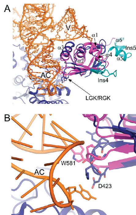
Figure 6. Model of tRNA Tyr binding by the An mt TyrRS C-terminal domain. (A) Superposition of the An mt TyrRS C-terminal domain (magenta/cyan) on the Tt TyrRS cocrystal structure 11 (blue, orange). Unordered residues preceding \beta 1 in the An mt TyrRS structure have been removed for clarity. (B) The RGK \beta -hairpin contacts the anticodon arm of tRNA Tyr . Residues 420–RGKD–423 from Tt TyrRS and the equivalent residues (578–LGKW–581) from the An mt TyrRS are shown as sticks. D423 of the Tt TyrRS is equivalent to W581 of the An mt TyrRS. Ac, anticodon arm; V, variable arm.
