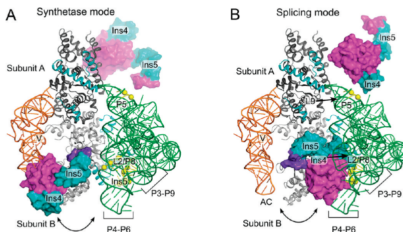
Figure 7. The An mt TyrRS C-terminal domain must undergo a large shift on the flexible linker to bind tRNA Tyr and a group I intron RNA on opposite sides of the catalytic domain. The figure shows the An mt TyrRS C-terminal domain (magenta, cyan) appended to the CYT-18/Δ424-669-Twort cocrystal structure 18 (gray, green) with tRNA Tyr (orange) from T. thermophilus cocrystal structure. 11 (A) Model for tRNA-binding (synthetase) mode. The An mt TyrRS C-terminal domain is positioned to match that of the Tt TyrRS in the Tt TyrRS-tRNA Tyr cocrystal structure. 11 (B) Model for group I intron-binding (splicing) mode. The An mt TyrRS C-terminal domain is positioned to satisfy distance restraints from site-directed hydroxyl radical cleavage experiments in which EPD-Fe conjugated at CYT-18 positions G423C and C424 (G529 and A530 in the An mt TyrRS; not visible in this view) cleaved the bound Nc ND1 intron at P3[5'] bp 3–4; P6[3'] bp 3; J6/6a[3'] nt 1; P6a[5'] bp 1–3; P6a[3'] bp 1; P8[3'] bp 4–5, and P5[5'] bp 3–4 (ref 19 and Paukstelis, Coon, and Lambowitz, unpublished data). The yellow spheres show the cleaved group I intron backbone phosphate positions in the Twort intron. Pezizomycotina-specific Ins4 and Ins5 are in cyan. Ins3 is not shown.
