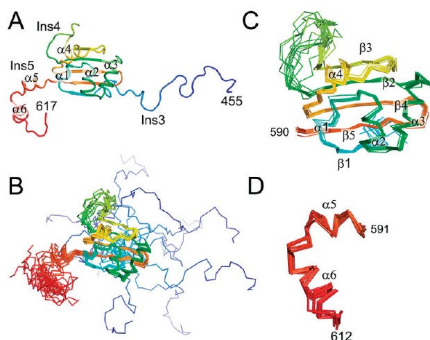
Figure 3. NMR structure of the An mt TyrRS. (A) Cartoon diagram of a representative structure from the NMR ensemble. (B) Superposition of 12 structures of the C-terminal domain of the A. nidulans mt TyrRS that satisfy the NMR-derived constraints equally well. The positions of the \beta -strands and \alpha -helices that form the core of the S4 fold are well-defined by the NMR data, while the locations of the termini and the loop of Ins4 between \beta 2 and \beta 3 are less certain. (C) Superposition of residues 490–590 from the 12 structures showing that the core of the S4 fold is well-defined by the NMR constraints. (D) Superposition of \alpha 5 and \alpha 6 of Ins5 from the 12 structures showing that the positions of these two helices are well-defined relative to each other, although their positions relative to the rest of the domain are not as well-defined (panel B). The color is ramped blue to red from the N- to C-terminus.
