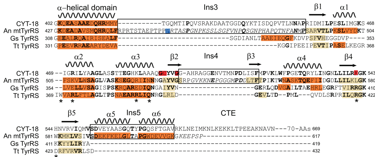
Figure 2. Structure-based sequence alignment of the Nc mt TyrRS (CYT-18) and An mt TyrRS with the Gs and Tt TyrRS C-terminal domains. The alignment begins with the last helix of the intermediate \alpha -helical domain. Secondary structural elements in the An mt TyrRS C-terminal domain are shown at the top, and \alpha -helices and \beta -strands observed in NMR or X-ray crystal structures (this work and refs 9 and 11) are highlighted in orange and beige, respectively, in the alignments. Residues in bold are conserved in two or more of the aligned proteins, and residues in italics are flexible in the An mt TyrRS C-terminal domain NMR structure based on ^{15}\text{N} relaxation. The blue highlighted residue in the An mt TyrRS (P455) is the first residue in the NMR construct whose structure is described here, and red highlighted residues in CYT-18 are those that were EPD-Fe conjugation sites in site-directed hydroxyl radical cleavage experiments (see Figures 7 and 8). Asterisks below the Tt TyrRS sequence indicate amino acid residues that contact tRNA Tyr in the cocrystal structure. 11 The boundaries of the Pezizomycotina-specific insertions are redefined relative to those in ref 2 based on the structural alignment.
