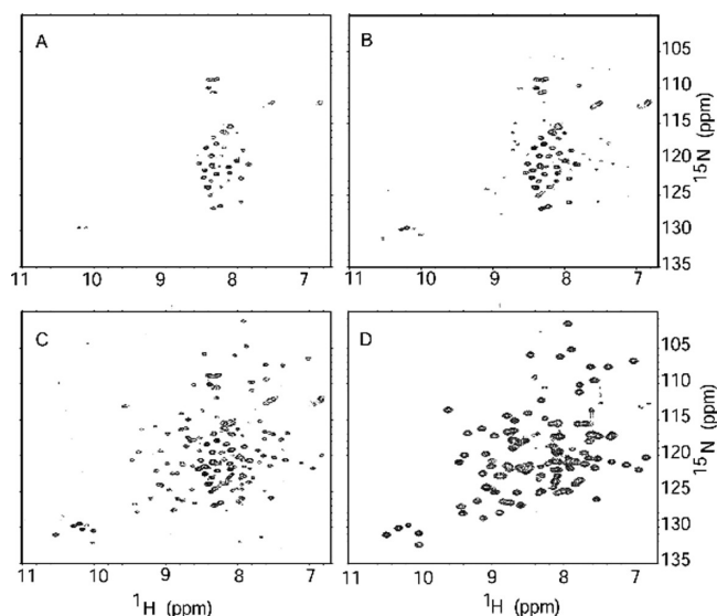
Figure 5. A time series of two-dimensional ^{15}\text{N} – ^1\text{H} spectra of the full-length An mt TyrRS. The resonances of the free C-terminal domain appear as the protein degrades. Spectrum A was acquired soon after sample preparation, spectrum B after \sim 10 h, and spectrum C after 24 h. Spectrum D is that of the purified C-terminal domain for comparison. The lack of observable resonances from the C-terminal domain within the intact full-length protein indicates that the tumbling of the C-terminal domain is restricted while it is part of the full-length protein.
