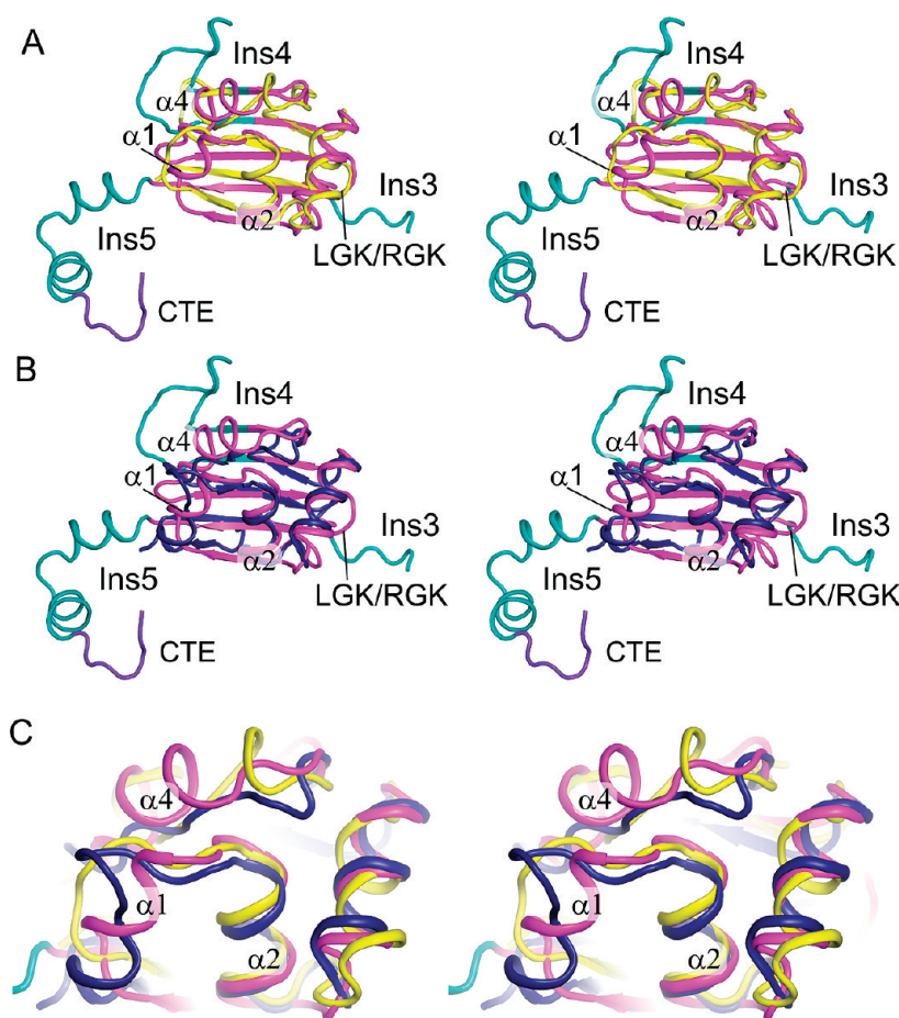
Figure 4. The An mt TyrRS C-terminal domain structure is similar to that of bacterial TyrRSs. (A) Stereoview superposition of the An mt TyrRS C-terminal domain NMR structure (magenta/cyan/purple) with that of the Gs TyrRS C-terminal domain (yellow; 8 ). (B) Stereoview superposition of the An mt TyrRS C-terminal domain with the Tt TyrRS C-terminal domain (blue) from the cocrystal structure with tRNA Tyr . 11 (C) Magnified view of \alpha -helical bundle region of the An mt TyrRS C-terminal domain with superposed bacterial TyrRS structures. \alpha 1 differs from the shorter helical region in the Tt TyrRS and is not present in the Gs TyrRS, and \alpha 4 is not present in either of the bacterial TyrRSs.
